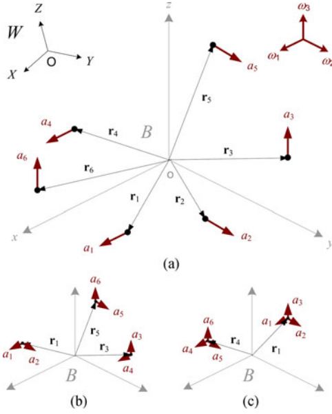
Fig. 2. Three different arrangements of six one-axis acceleration measurements. (a) Six one-axis measurements at six distinct locations. (b) Three two-axis measurements at three distinct locations. (c) Two three-axis measurements at two distinct locations.
